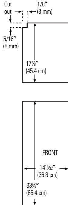
Freezer Panel With Dispenser
